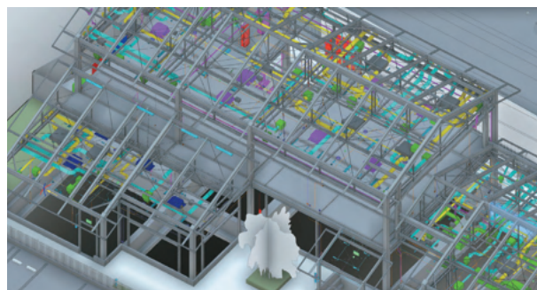
Clash detection using BIM
