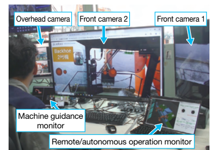
Construction status using remote-controlled/autonomous operation system
